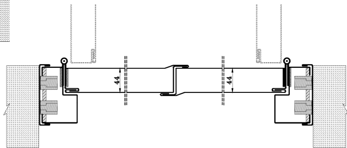
Fig. 3 Double door with single rebate frame assembly
