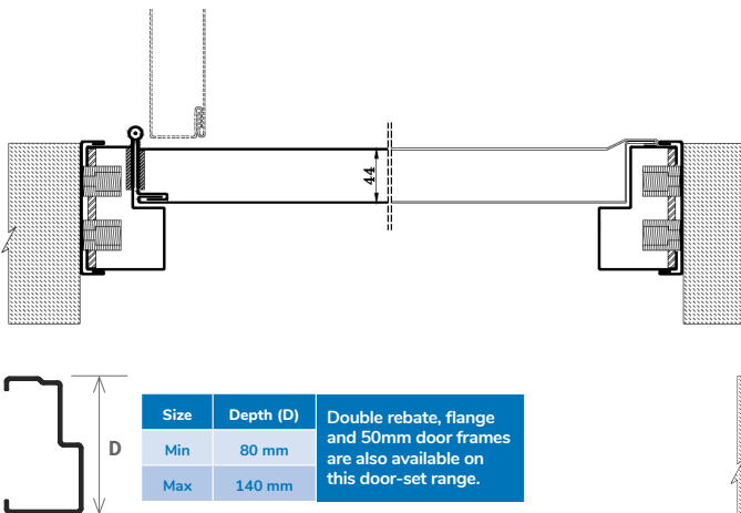
Fig.1 Single door with single rebate frame assembly
