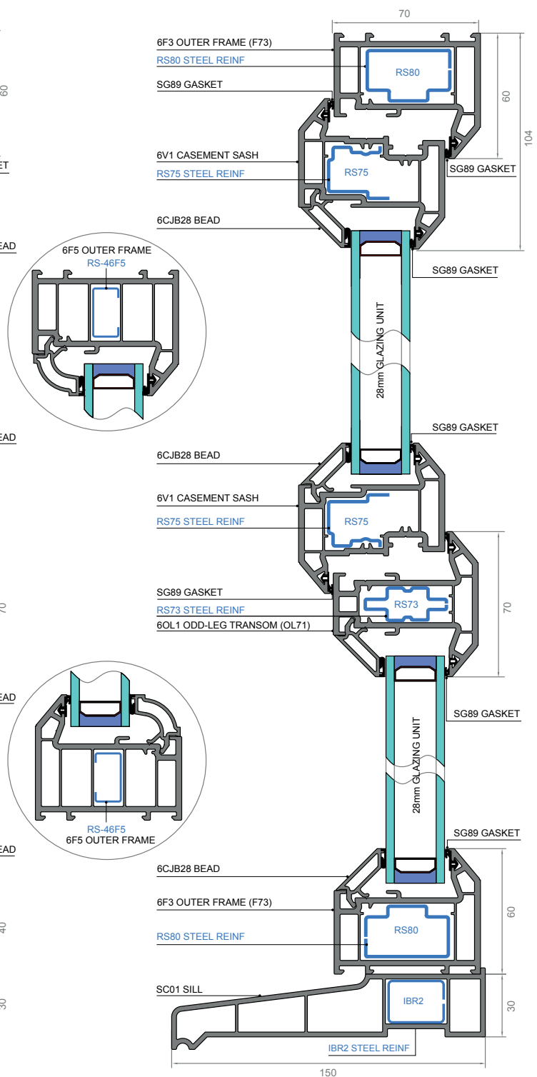
Externally beaded with intermediate outer frame, chamfered j bead and steel reinforcements
