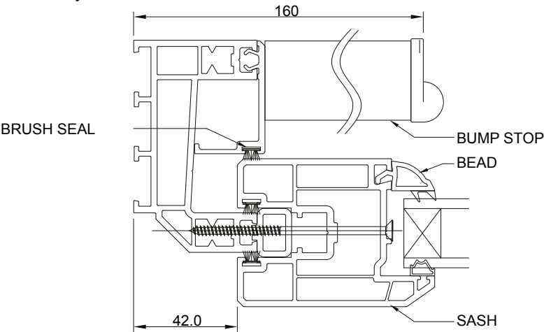
Assembly Section C
