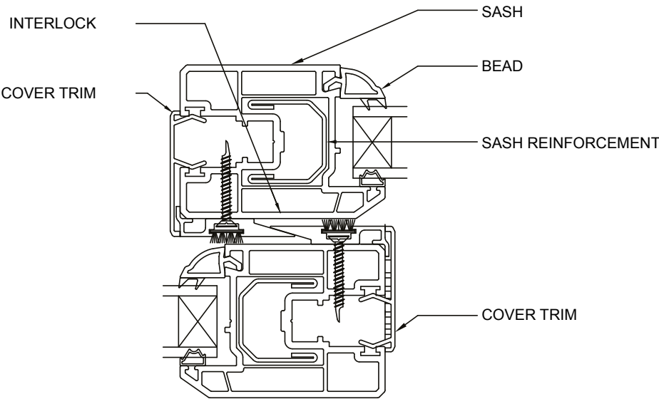
Assembly Section D
