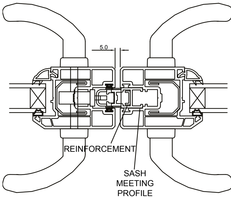
Assembly Section N
