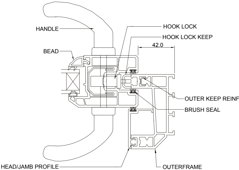
Assembly Section E
