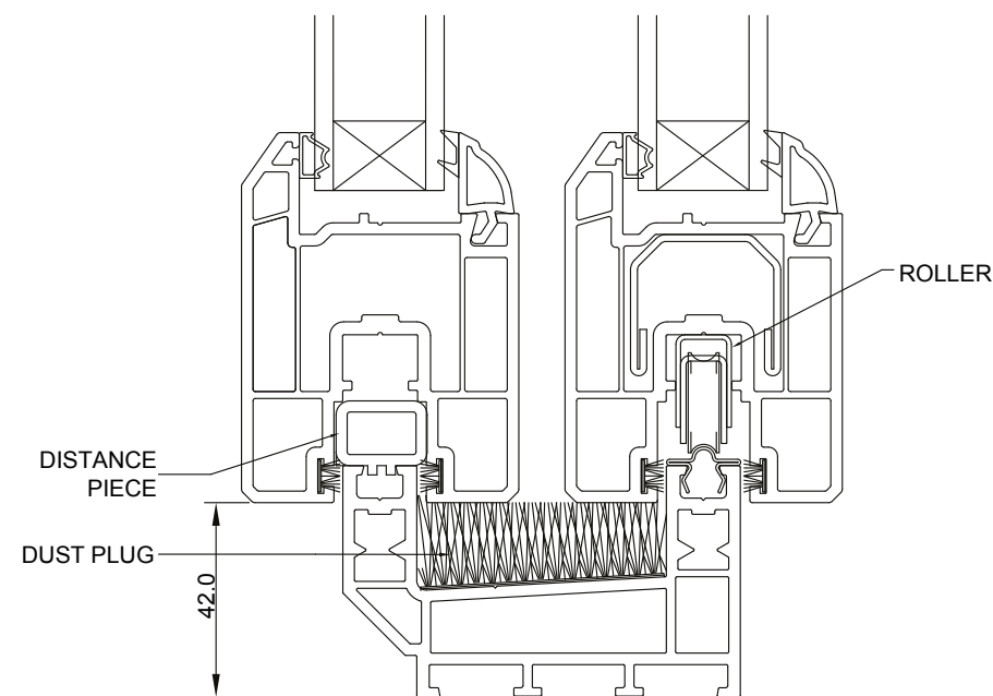
Assembly Section G
