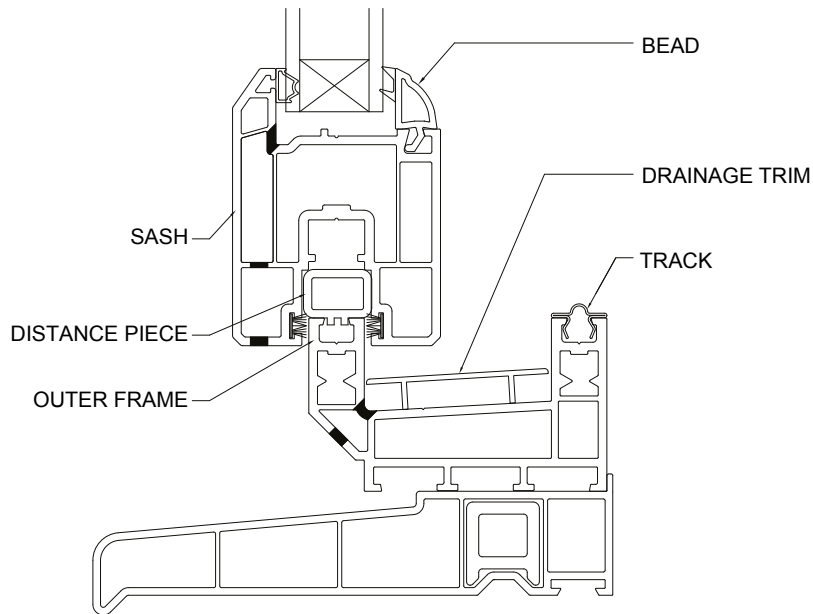
Assembly Section L
