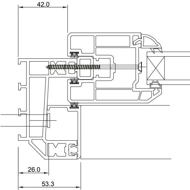
Assembly Section J
