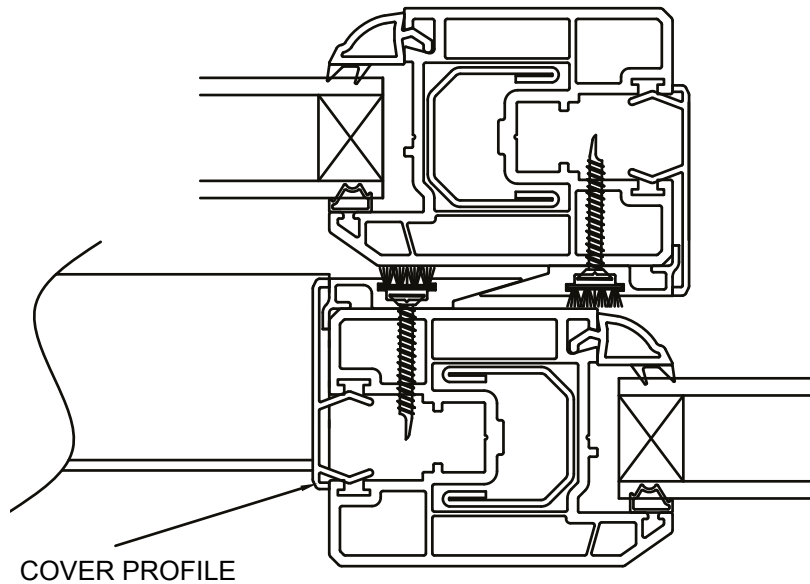
Assembly Section M
