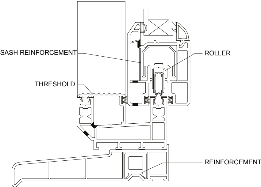
Assembly Section H
