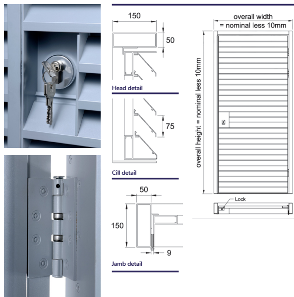
Single door
