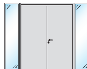
Glazed side-panels
