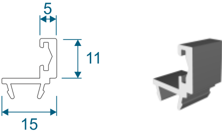
VS041 - Wool Pile Carrier
