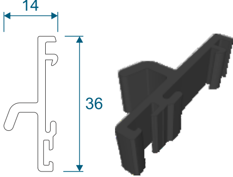
VS052 - Travel Stop
