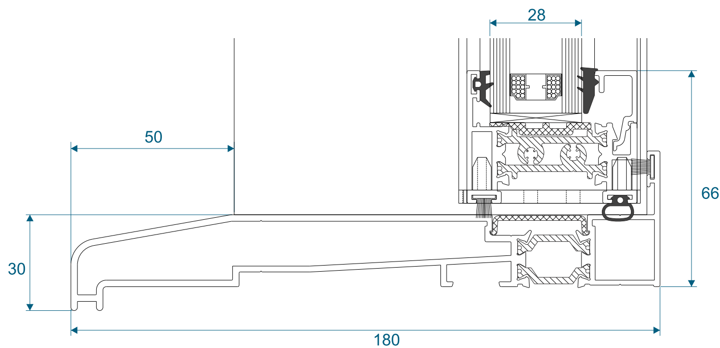
With Slim Bottom Rail
