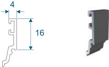
VS046 - External Bead
