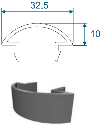
VS052 - Travel Stop
