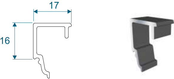
VS046 - External Bead
