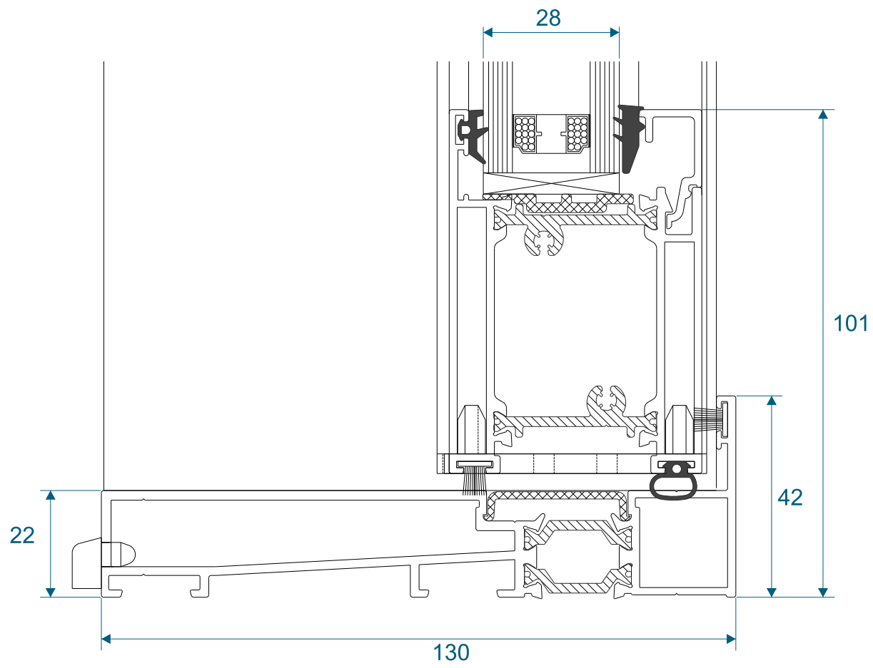
With Deep Bottom Rail
