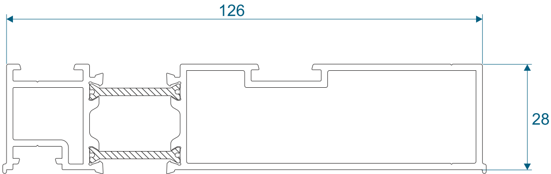
VS011 - Head Frame
