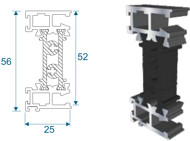
VS124 - Vertical Member
