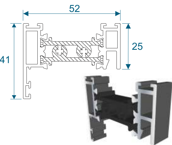
VS020 - Top & Bottom Rail
