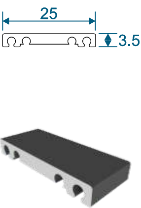
ZSB246 - 25mm Flat Astragal
